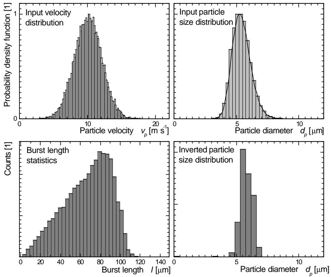
Fig. 5: Example of a simulated polydispersed spray and the estimated particle size distribution from the burst-length statistics.
