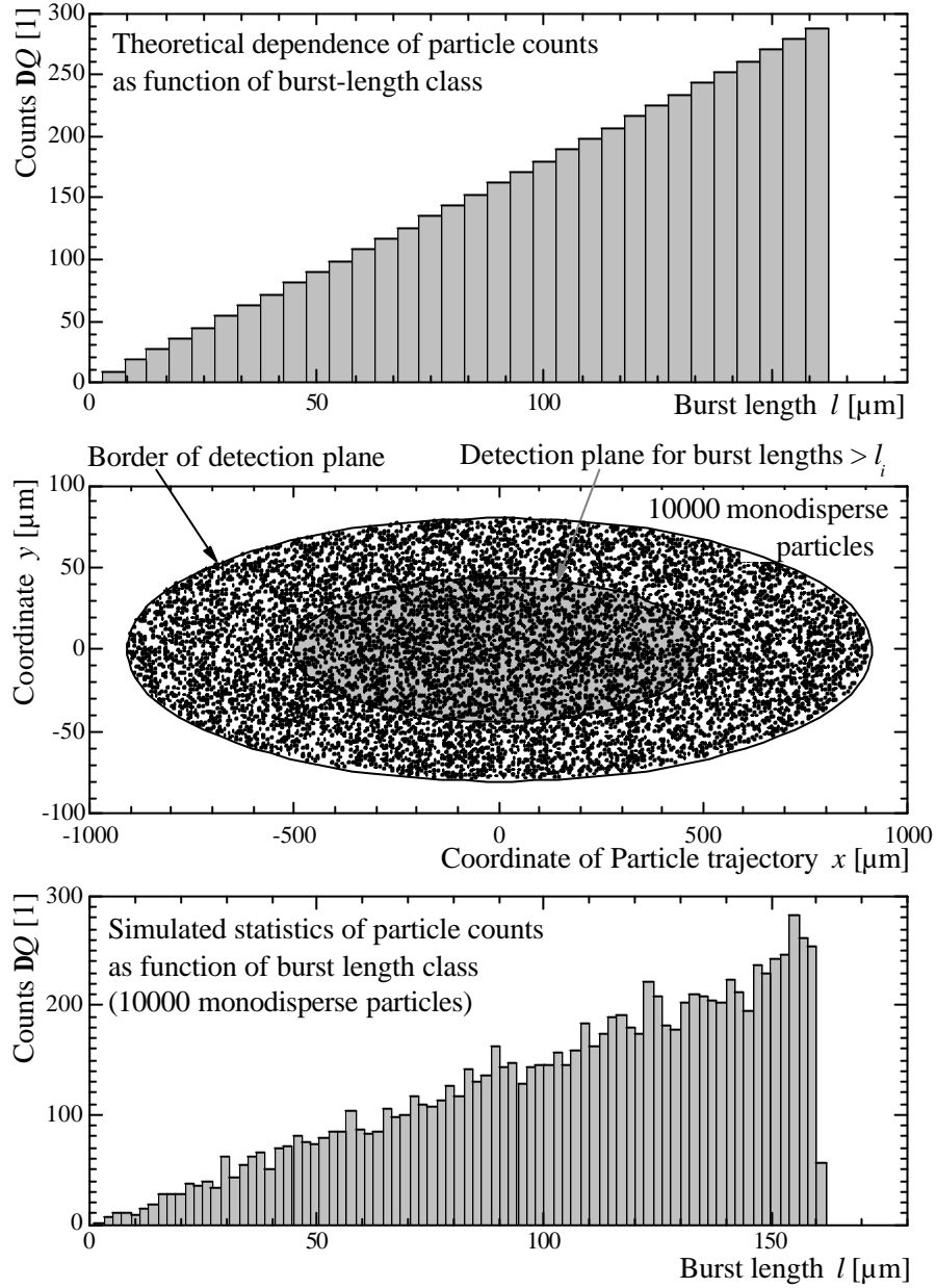
Fig. 1: Burst-length statistics for monodisperse particles. a) Theoretical dependence, b) Simulated statistical particle trajectories, c) Statistical burst-length distribution.
