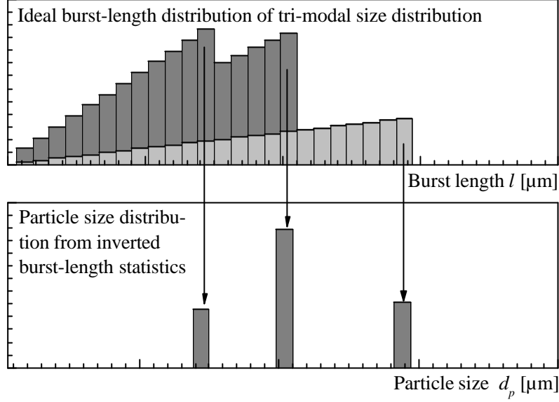
Fig. 2: Ideal burst-length statistics of a tri-modal particle size distribution and their statistical inversion.
