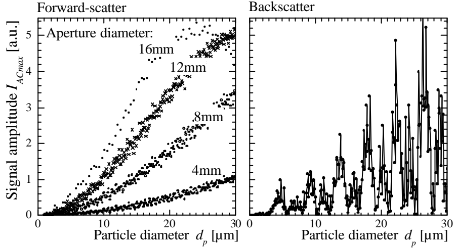
Fig. 3: Maximum modulated signal intensity as a function of the particle diameter. a) Forward scatter configuration with a nearly monotonic relation, b) Backscatter configuration exhibiting strong oscillations.
