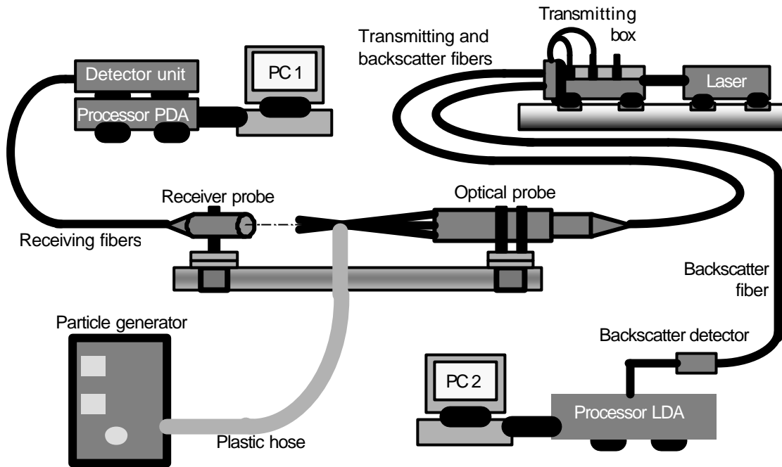
Fig. 7: Experimental setup
