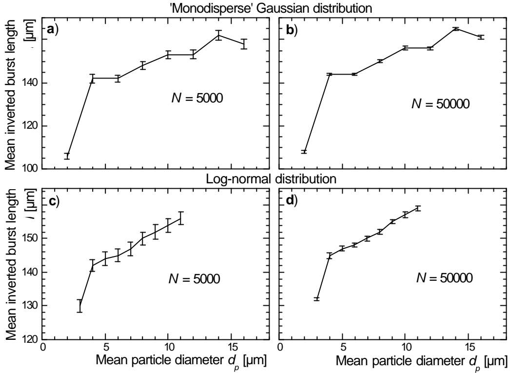
Fig. 6: Estimated mean inverted burst length and its variance for different number of samples as a function of the mean diameter of 'monodispersed' and log-normal particle size distributions.
