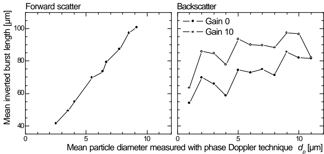
Fig. 8: Measurements of 'monodispersed' Gaussian particle size distributions. The mean inverted burst length is shown for forward and backscatter measurements.
