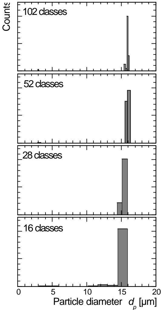
Fig. 4: Computed particle size distributions using various numbers of size classes.
