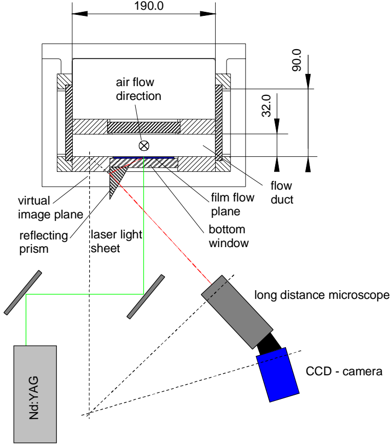
Fig. 2: Experimental setup of the PIV system for film flow investigations
