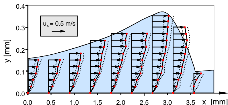
Fig.1: Velocity profiles inside a shear driven liquid film, combined by matching simultaneous film thickness and velocity measurements.
