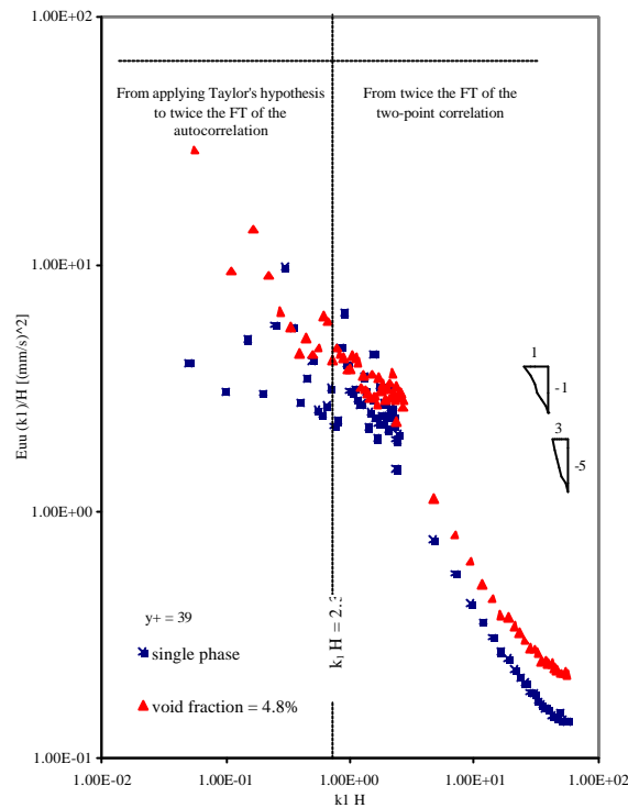
Fig.4 dimensional spectra of the streamwise fluctuating velocity at y/H = 0.121
