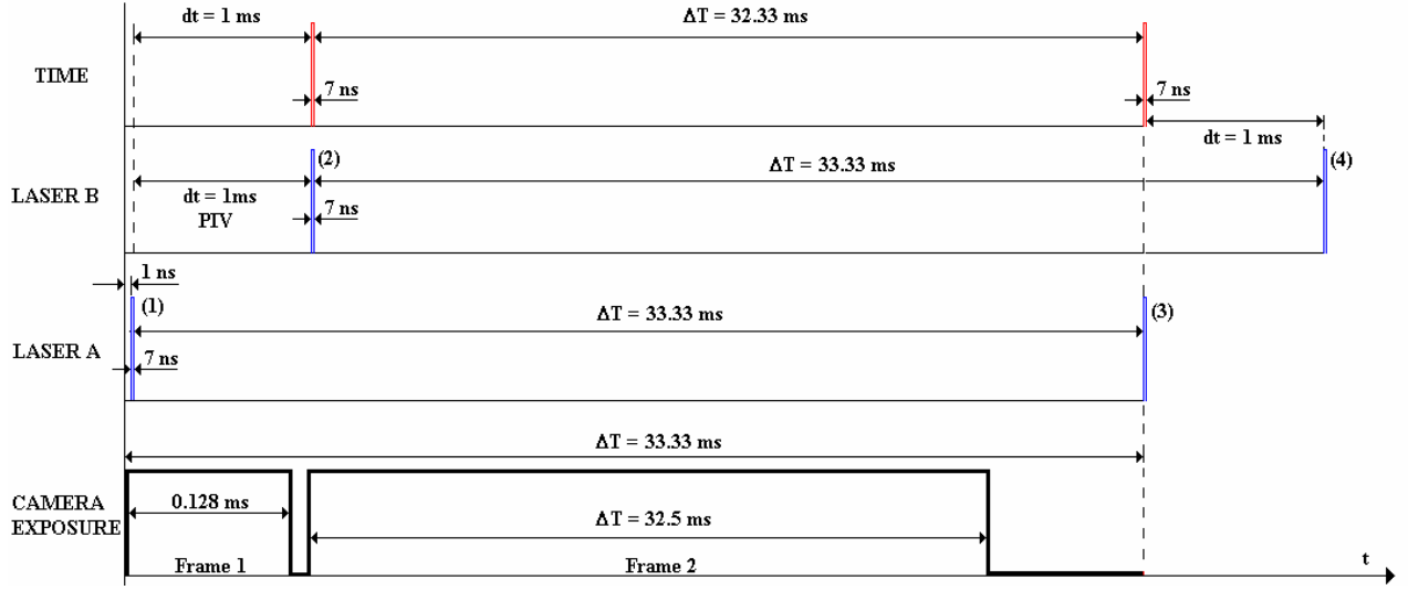
Fig. 2. Synchronization diagram
