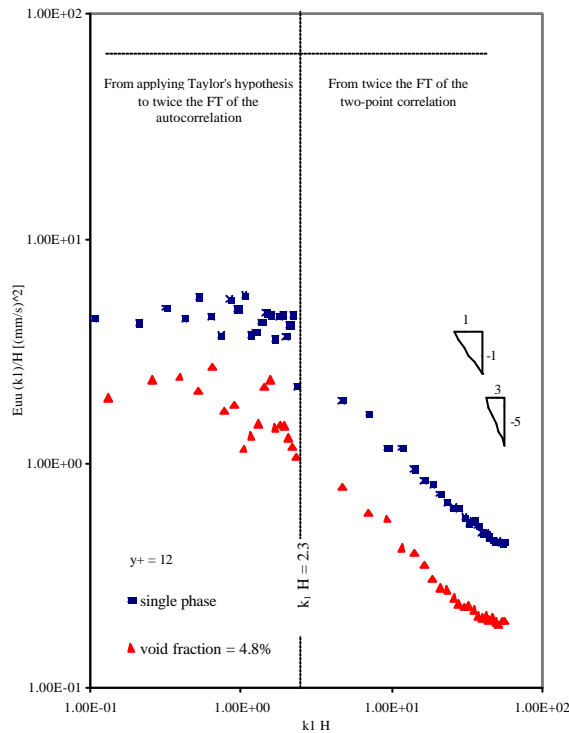
Fig. 3 dimensional spectra of the streamwise fluctuating velocity at y/H = 0.037
